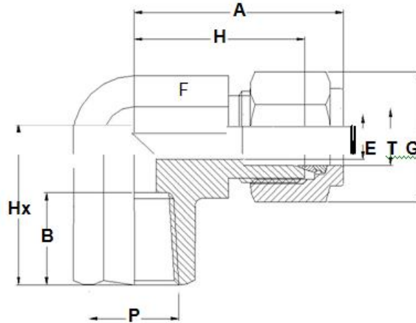
INCH OD Tubes X Female NPT Threads
